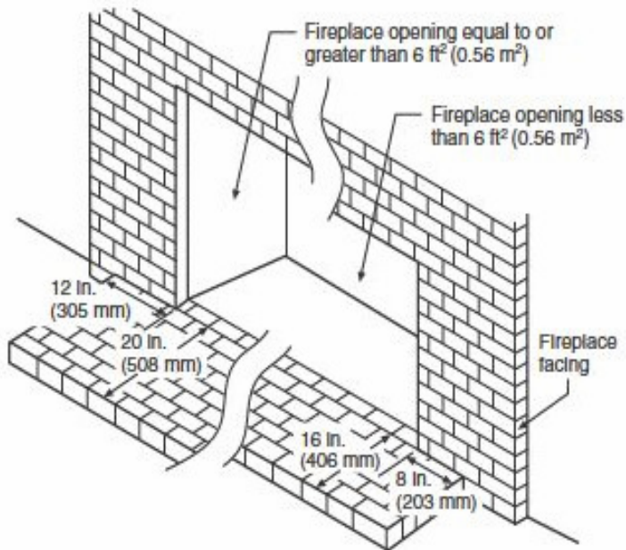
FIGURE 11.3.3 Fireplace Hearth Extension Requirements.
